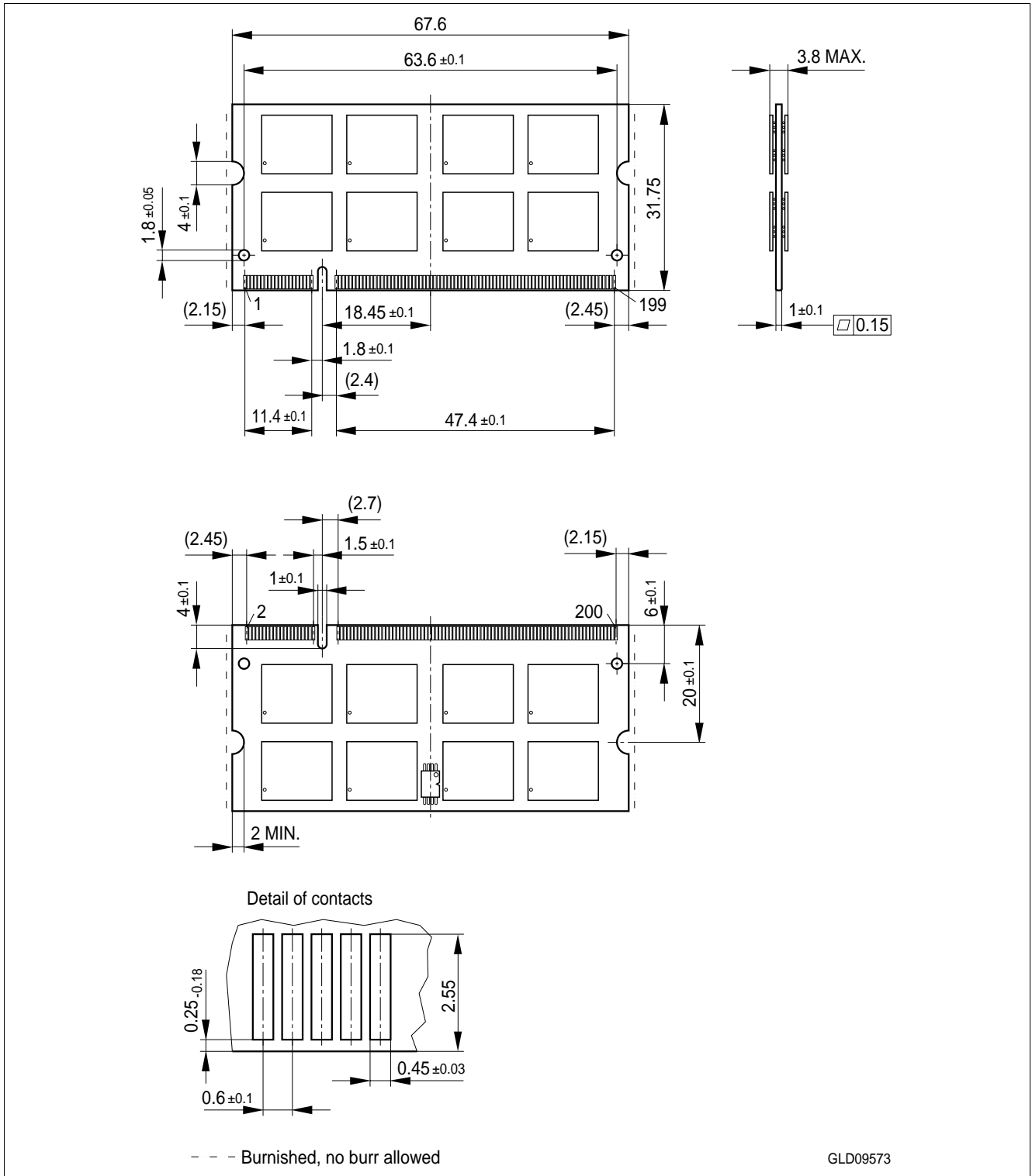
Figure 3 Package Outline SO-DIMM L-DIM-200-22
