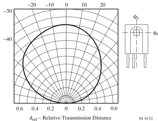
Figure 13. Vertical Directivity \phi_y
