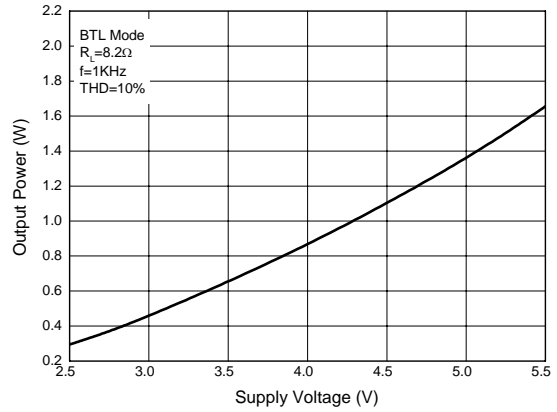
Figure 13. Output Power vs. Power Supply
