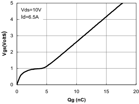
Figure 7: Gate-Charge Characteristics
