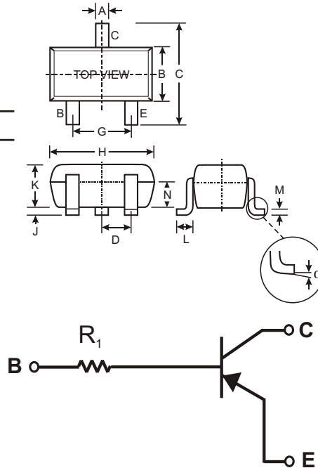
SCHMATIC DIAGRAM
