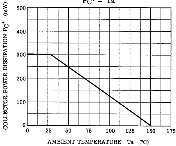
P_C^* - T_a
