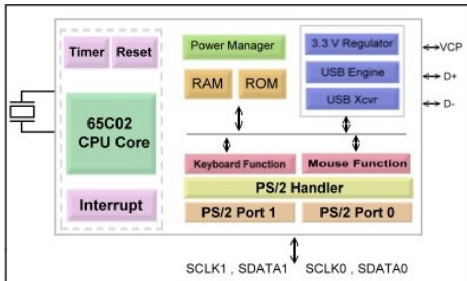
DataSheet4U.com CSC0101A Functional Block Diagram
