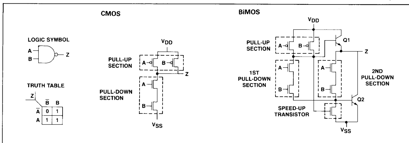
FIGURE 4 — CMOS/BiMOS 2-INPUT NAND COMPARISON
