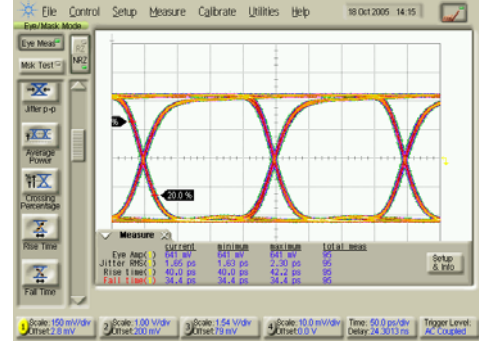
Bit rate: 5 Gb/s Vin = +/-10 mVpp, Vout = +/-650 mVpp
