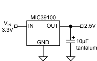
2.5V/1A Regulator
