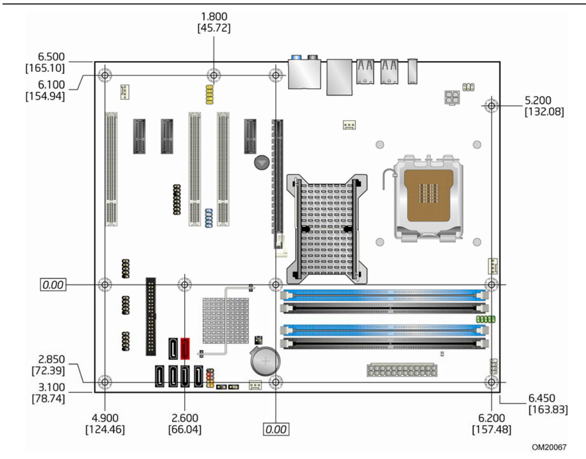
Figure 15. Board Dimensions
