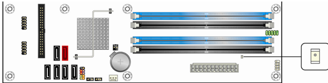
Figure 7. Location of the Standby Power Indicator LED
