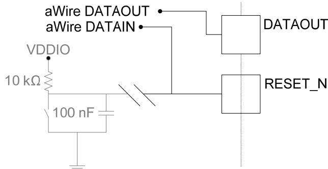
Figure 14-4. aWire with full-duplex communication.
