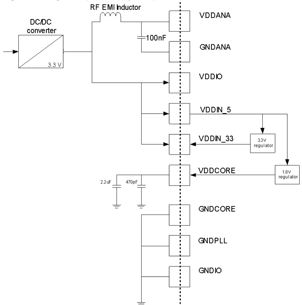
Figure 4-1. Single 3.3V power supply example schematic.
