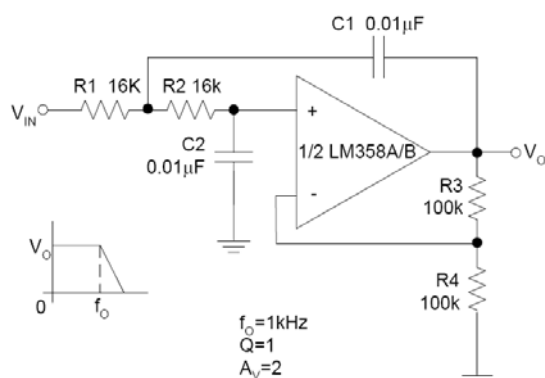
Fig.19- DC Coupled Low-Pass Active Filter
