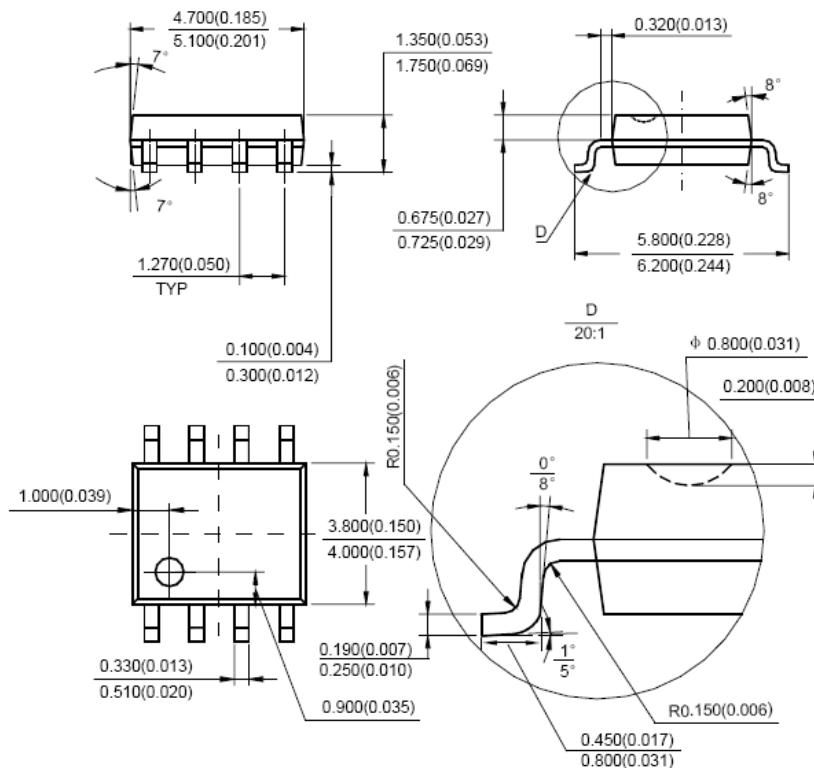
SOP-8
