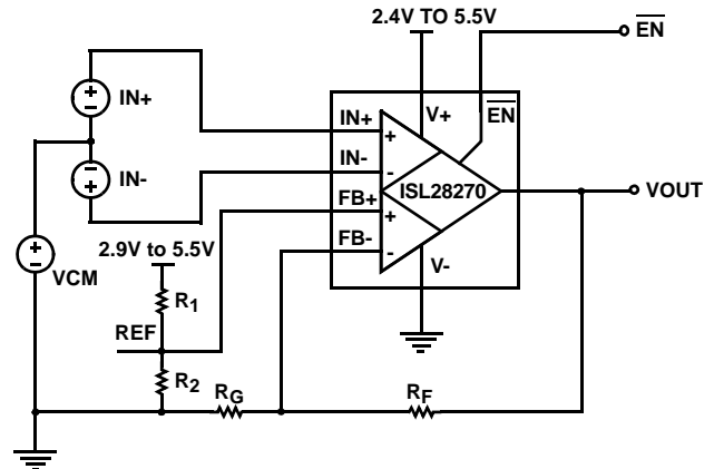
FIGURE 50. GAIN SETTING AND REFERENCE CONNECTION
