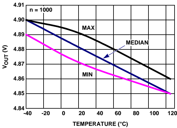
FIGURE 45. V_{OUT} HIGH vs TEMPERATURE, R_L = 1k , V_+ , V_- = \pm 2.5V
