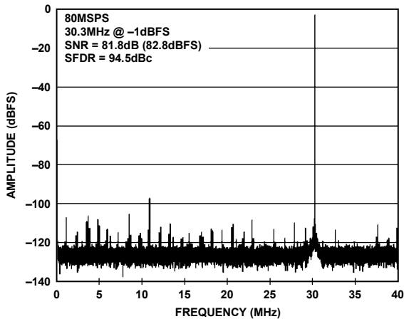
Figure 36. AD9650-80 Single-Tone FFT with f_{IN} = 30.3 MHz
