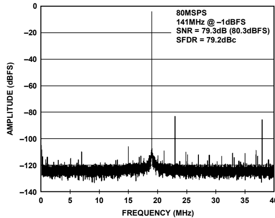
Figure 38. AD9650-80 Single-Tone FFT with f_{IN} = 141 MHz
