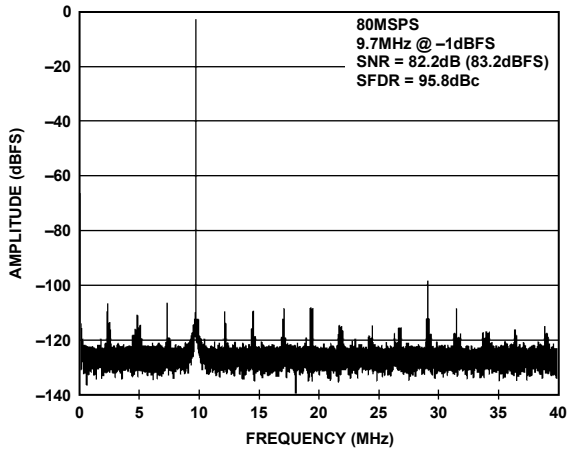
Figure 35. AD9650-80 Single-Tone FFT with f_{IN} = 9.7 MHz
