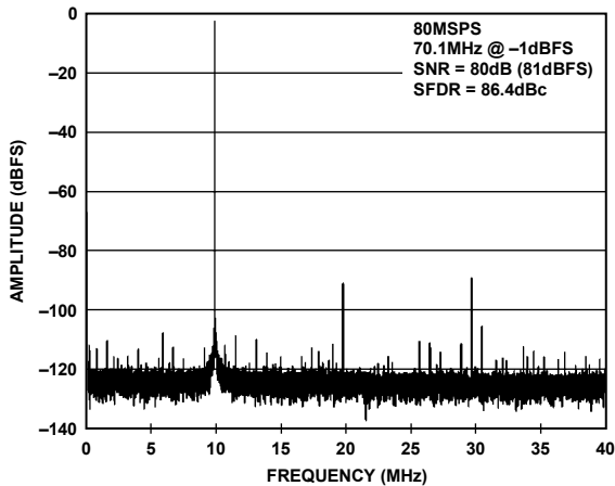
Figure 37. AD9650-80 Single-Tone FFT with f_{IN} = 70.1 MHz
