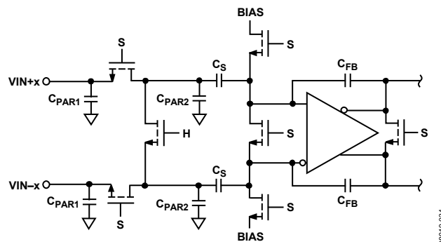
Figure 77. Switched-Capacitor Input
