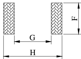
( PCB Pattern )
