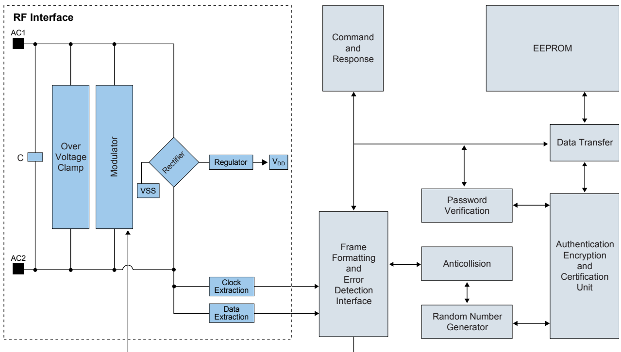
Figure 1. Block Diagram
