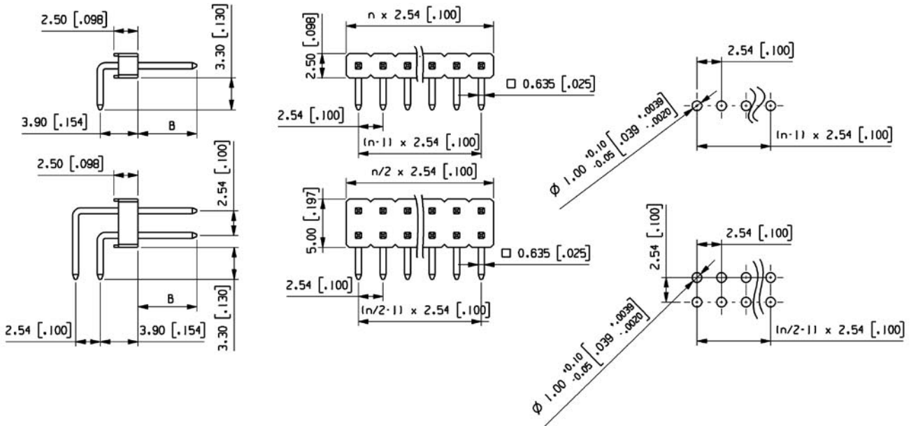
PCB Layout
