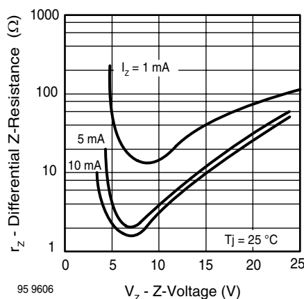
Figure 10. Differential Z-Resistance vs. Z-Voltage
