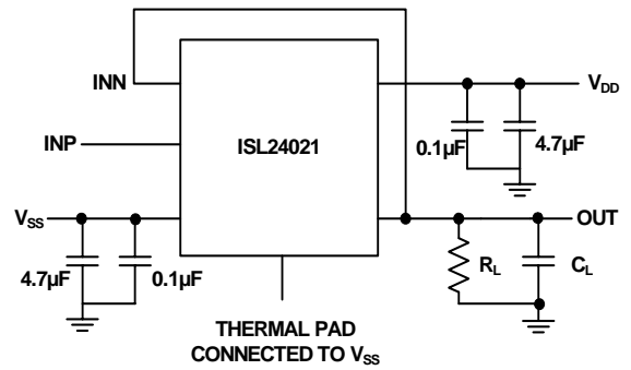
FIGURE 22. TEST CIRCUIT
