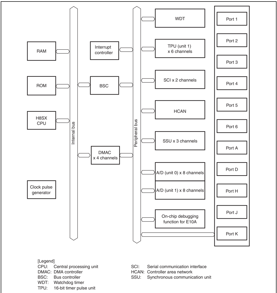
Figure 1.2 Block Diagram of H8SX/1525
