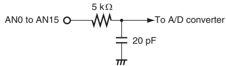
Figure 15.11 Analog Input Pin Equivalent Circuit
