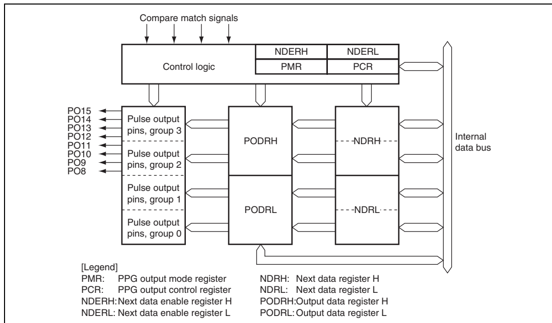
Figure 10.1 Block Diagram of PPG
