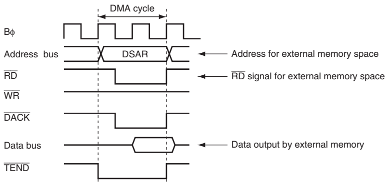
Transfer from external memory to external device with \overline{\text{DACK}}
