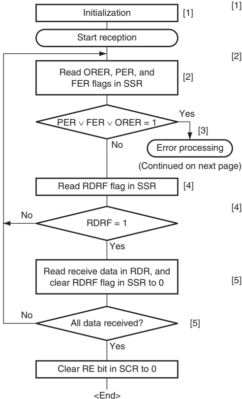
Figure 12.9 Sample Serial Reception Flowchart (1)
