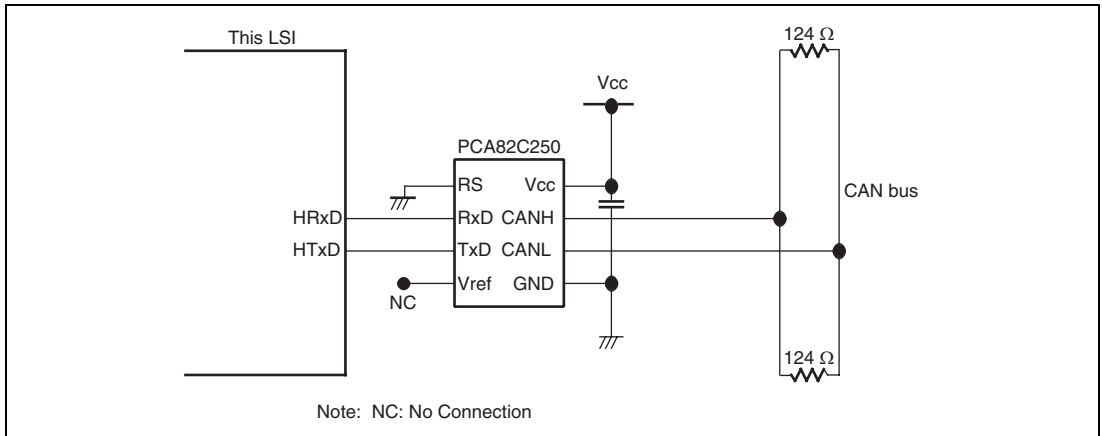
Figure 13.16 High-Speed Interface Using PCA82C250
