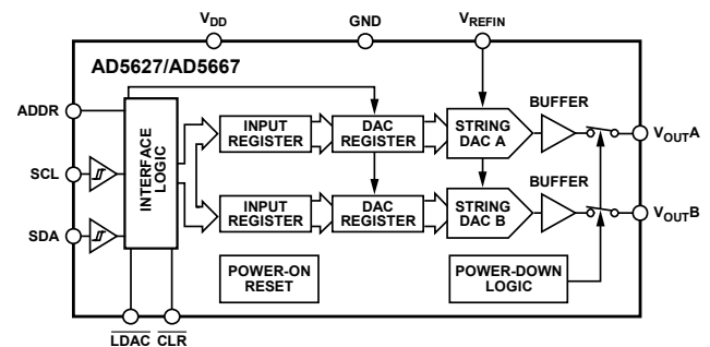
Figure 2. AD5627/AD5667
