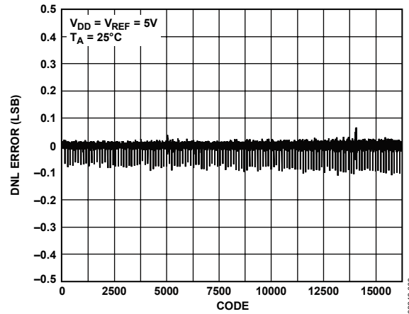
Figure 10. DNL AD5647R, External Reference
