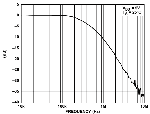
Figure 51. Multiplying Bandwidth
