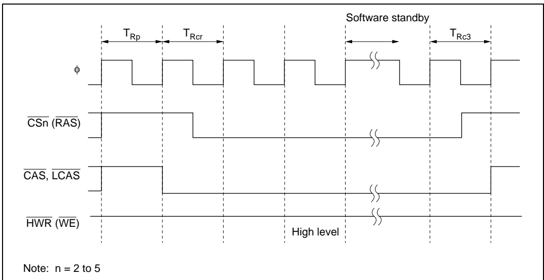
Figure 7.29 Self-Refresh Timing
