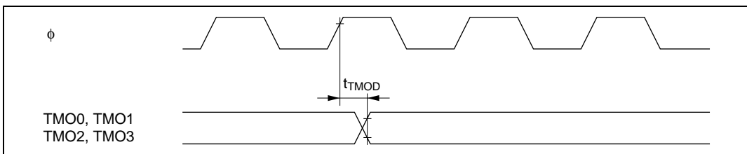
Figure 26.24 8-bit Timer Output Timing
