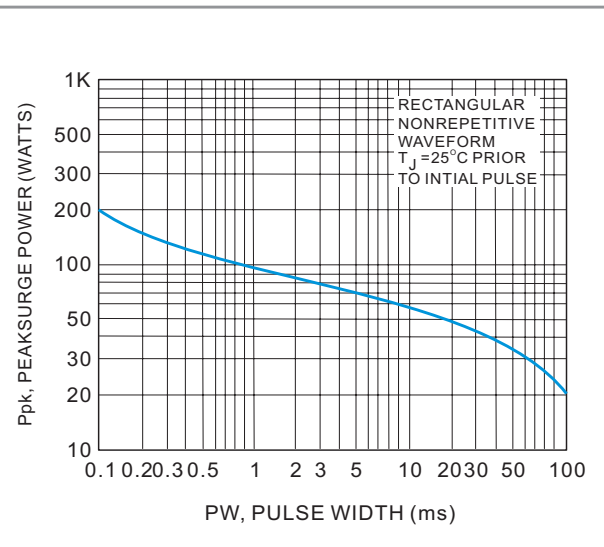
Fig. 6 Maximum Surge Power
