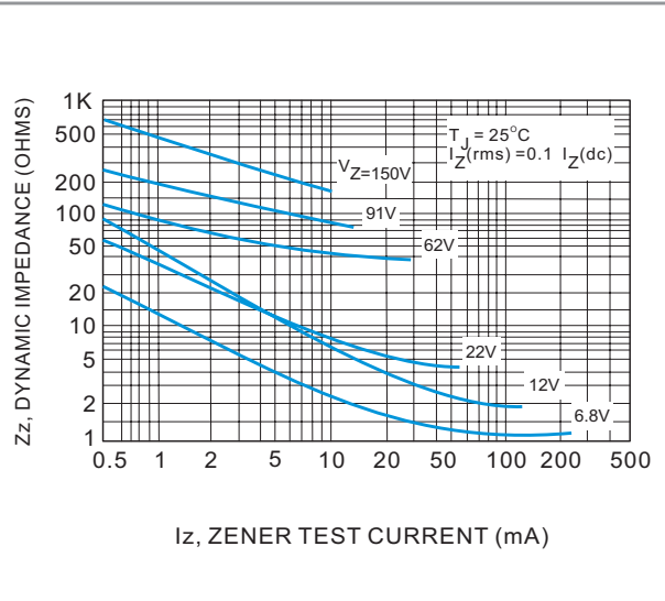
Fig. 4 Effect of Zener Current
