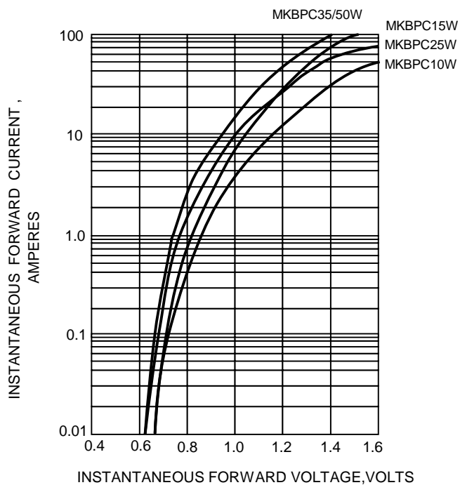
FIG.3-TYPICAL FORWARD CHARACTERISTICS
