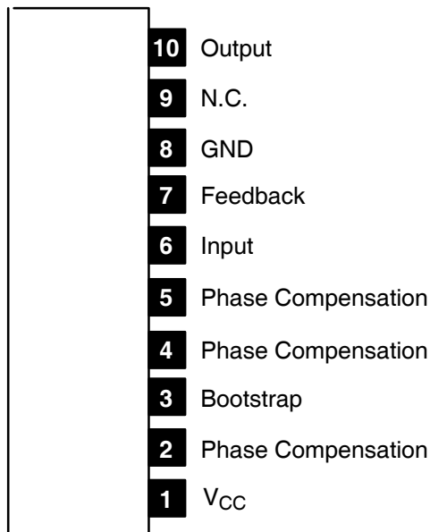
Pin Connection Diagram
