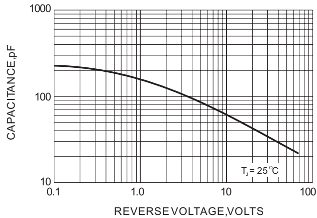
Fig.3-TYPICAL JUNCTION CAPACITANCE
