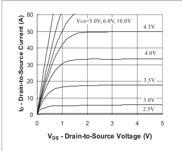
FIG.1- Output Characteristic
