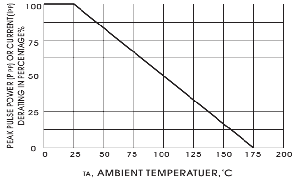
FIGURE 2-PULSE DERATING CURVE
