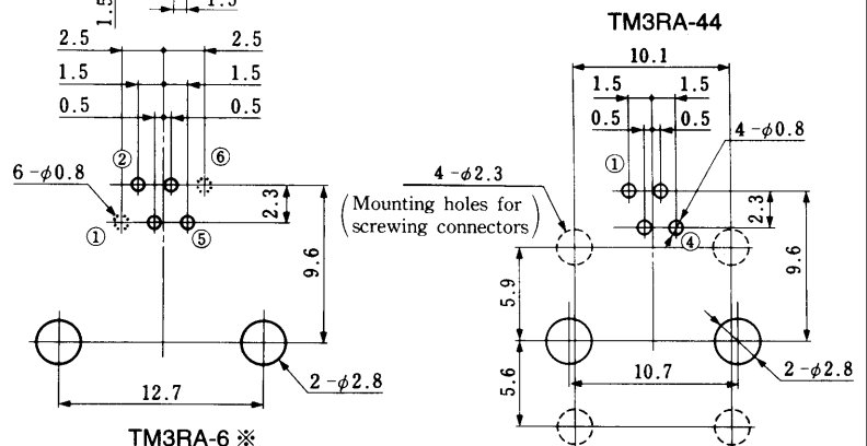
PCB mounting hole layout (Connector mounting side)
