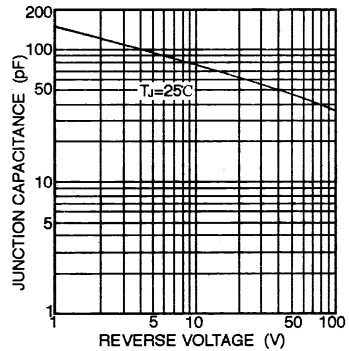
FIG. 4-TYPICAL JUNCTION CAPACITANCE
