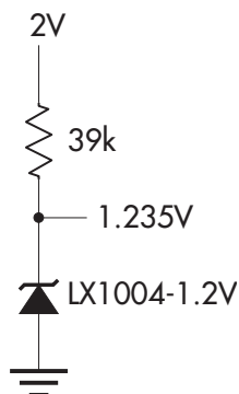
MICROPOWER REFERENCE FROM 2 CELL BATTERY
