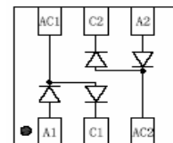
FBAT54SDW Marking:KL8
