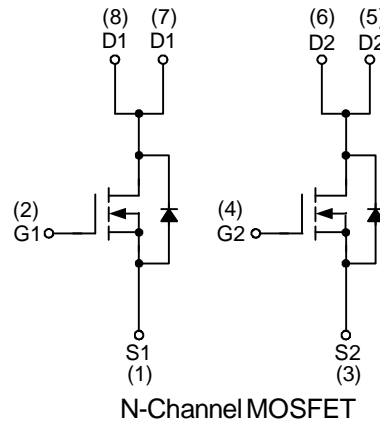
N-Channel MOSFET
