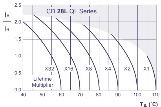
Lifetime Diagram
