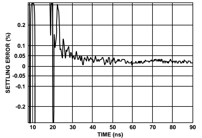
FIGURE 33. SETTLING RESPONSE
