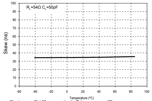
Driver Differential Skew vs Temperature
