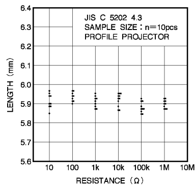
Fig.4 Dimensions (length)
