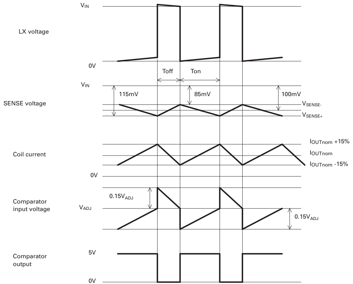
Figure 1 Operating waveforms
