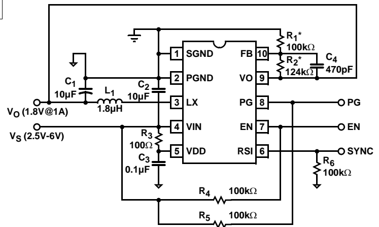
EL7531 TOP VIEW
