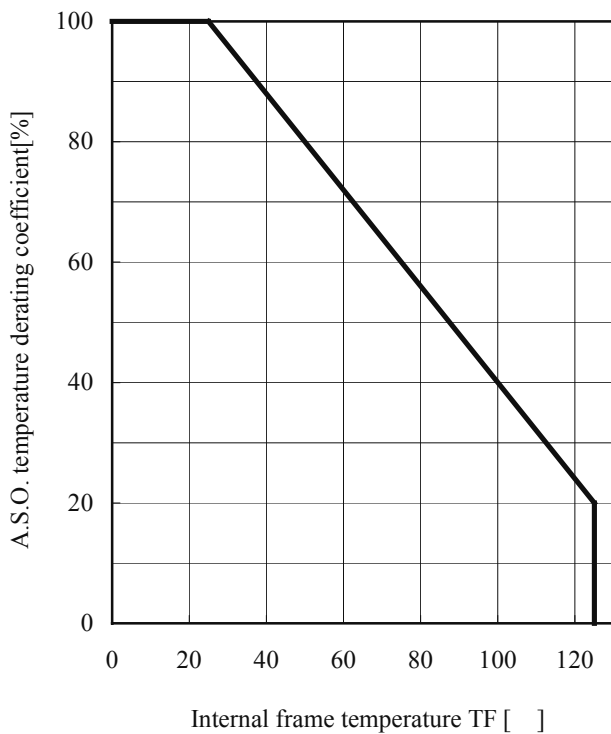
IRIS-X6757 A.S.O. temperature derating coefficient curve
