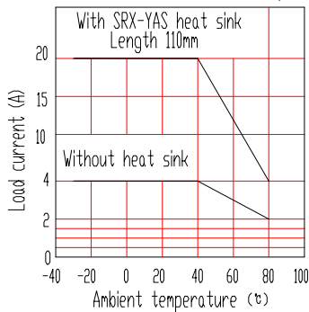
Load Current vs. Ambient Temp.
