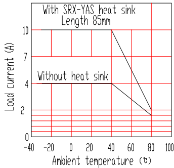
Load Current vs. Ambient Temp.
