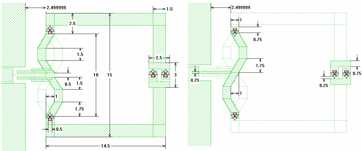
Fig. 2.3b. 915-868 MHz dual band cross tapped loop antenna, “small” type: top and bottom layer (top view) (dimensions in mm).
