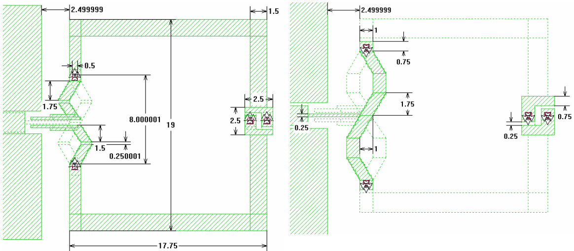
Fig. 2.4b. 915-868 MHz dual band cross tapped loop antenna, "big" type: top layer and bottom layer (top view) (dimensions in mm).
