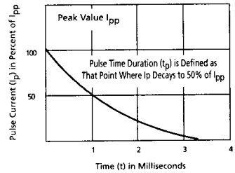
FIGURE 2 Pulse Waveform For Exponential Surge
