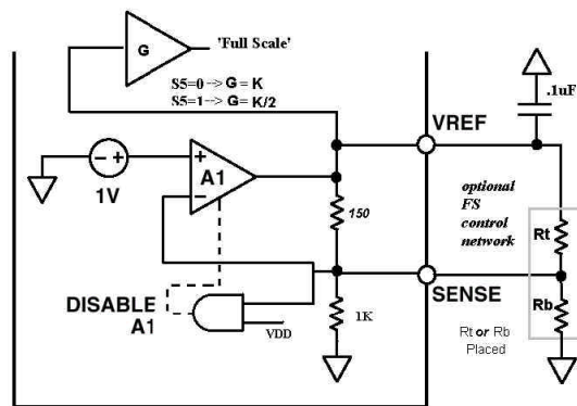
Simplified Voltage Reference Equivalent Circuit
