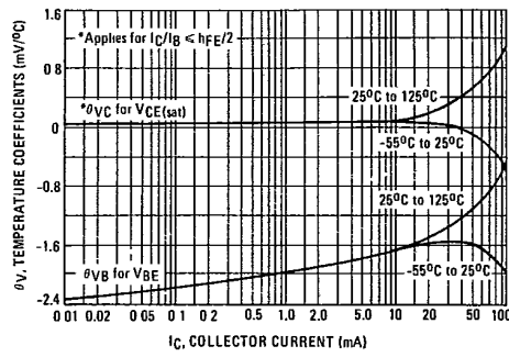
FIGURE 4 - TEMPERATURE COEFFICIENTS
