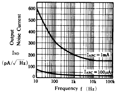
Output Noise Current vs. Frequency
