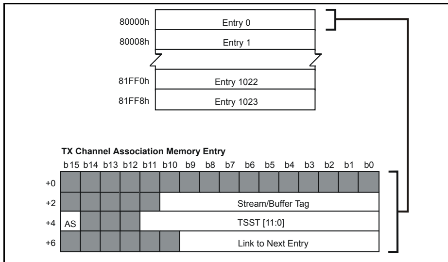
Figure 72 - TX Channel Association Memory
