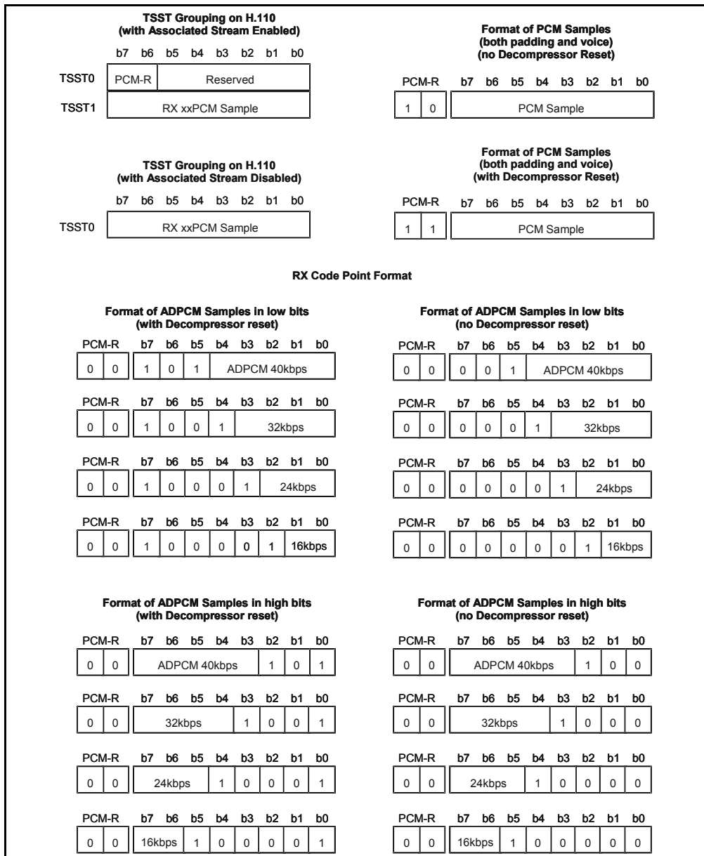
Figure 87 - Format of RX xxPCM TSSTs - 1 of 2
