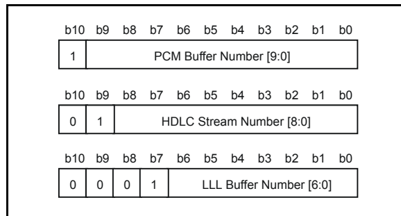
Figure 73 - Buffer Tag Format
