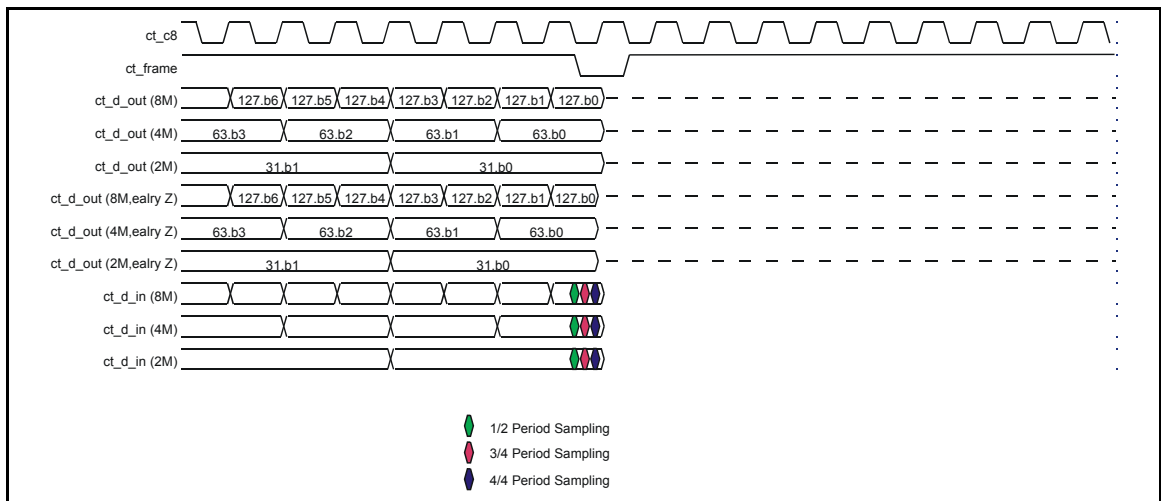
Figure 91 - TDM Bus Timing - ct_d
