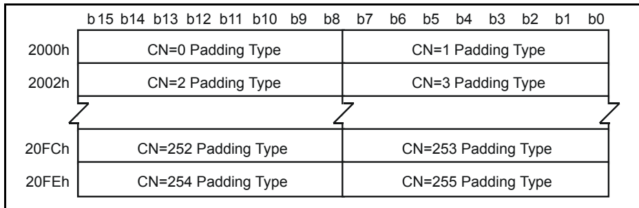
Figure 89 - CN Packet Conversion Lookup Table
