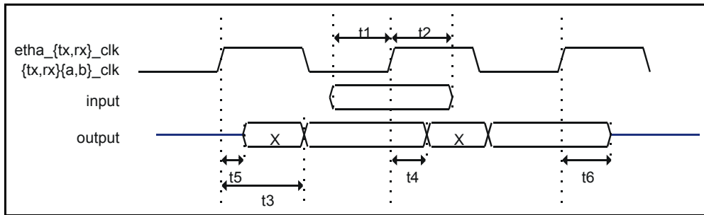
Figure 107 - UTOPIA / POS-PHY / Ethernet Timing
