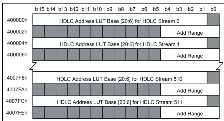
Figure 77 - HDLC Stream to HDLC Address LUT Structure
