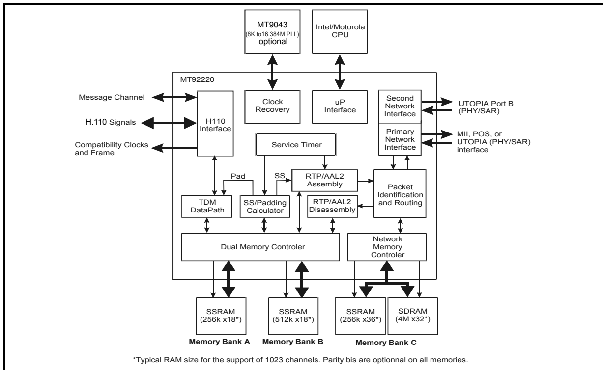
Figure 1 - MT92220 Block Diagram
