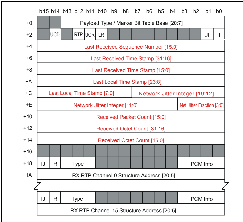
Figure 54 - RX RTP Connection Structure
