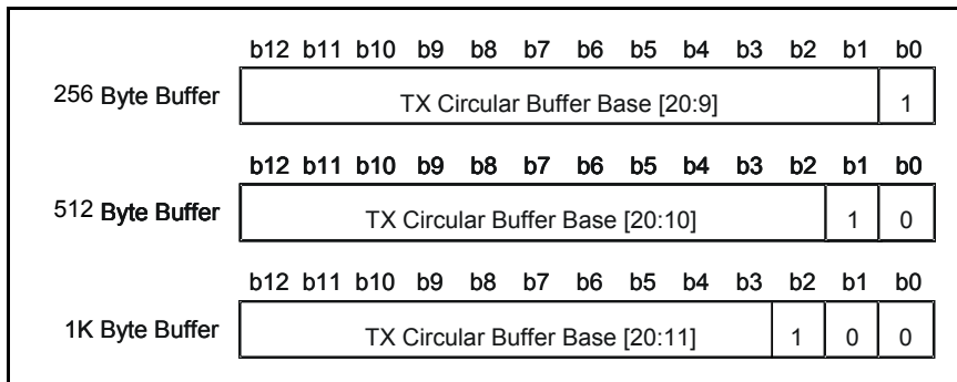
Figure 75 - TX Circular Buffer Base/Size Indication
