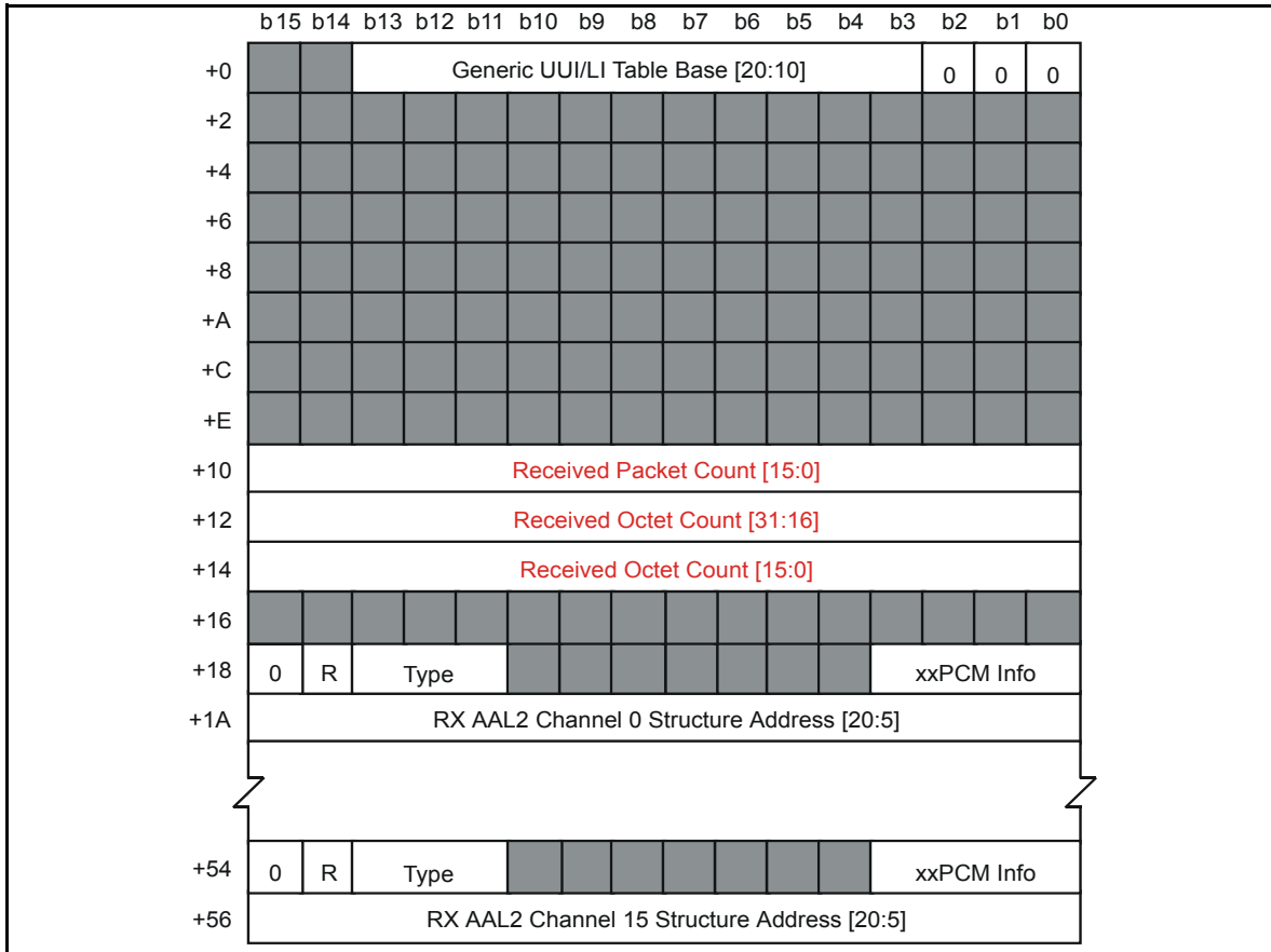
Figure 57 - RX AAL2 Connection Structure
