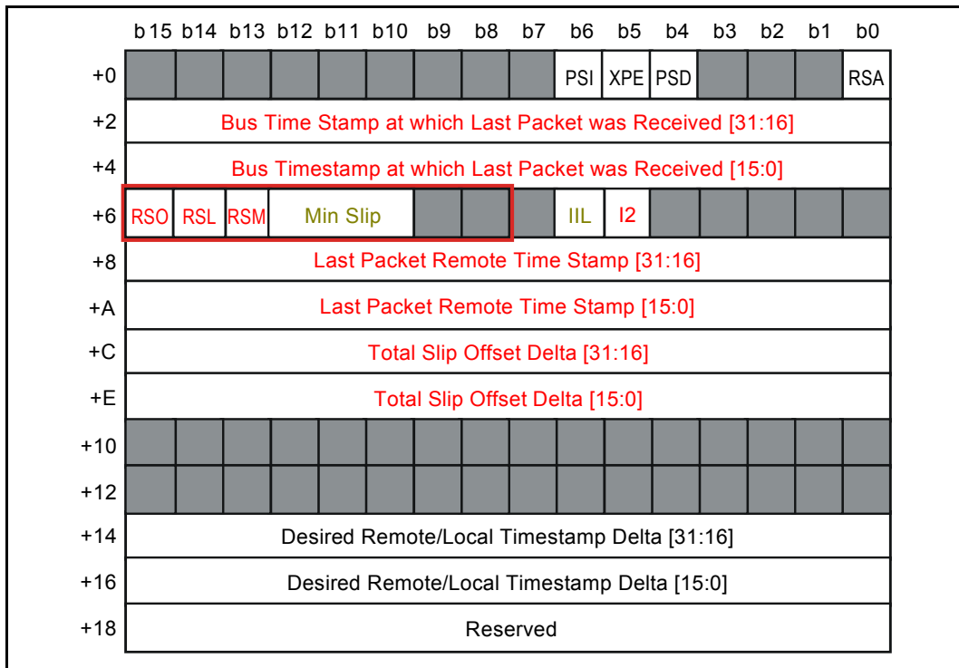
Figure 63 - RTP Common PDV Absorption Structure
