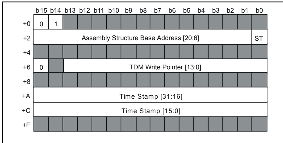
Figure 40 - Assembly Event - Service xxPCM RTP Channel
