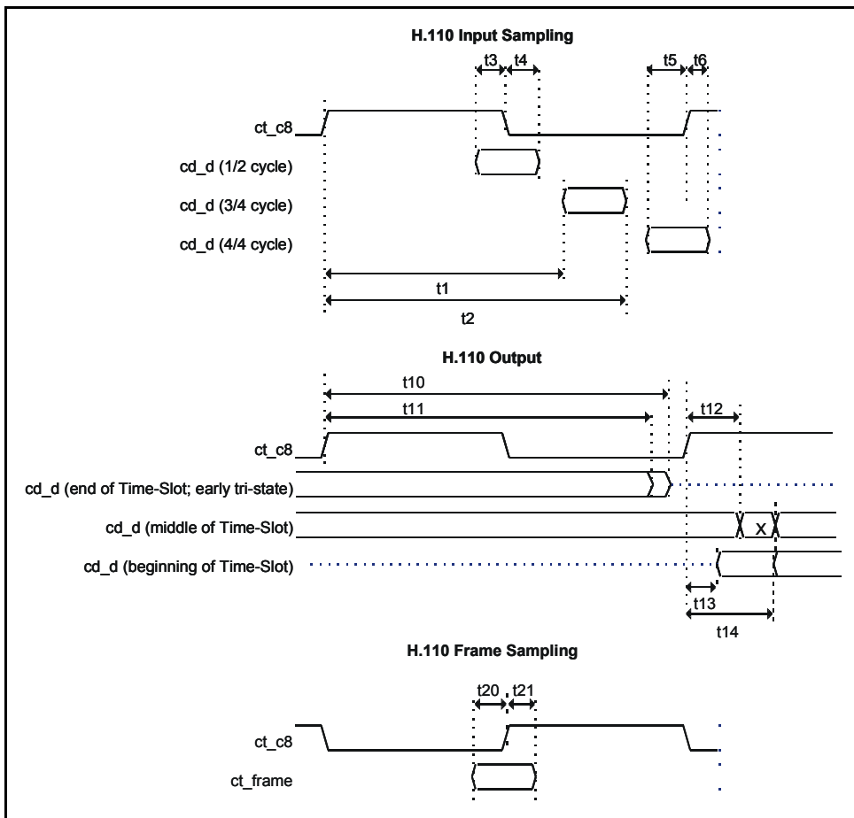
Figure 108 - H.110 Input Output
