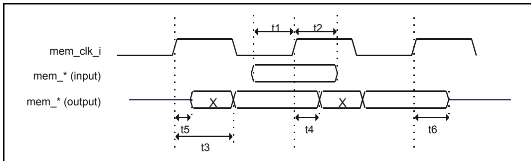
Figure 110 - External Memory Timing (both SSRAM and SDRAM)
