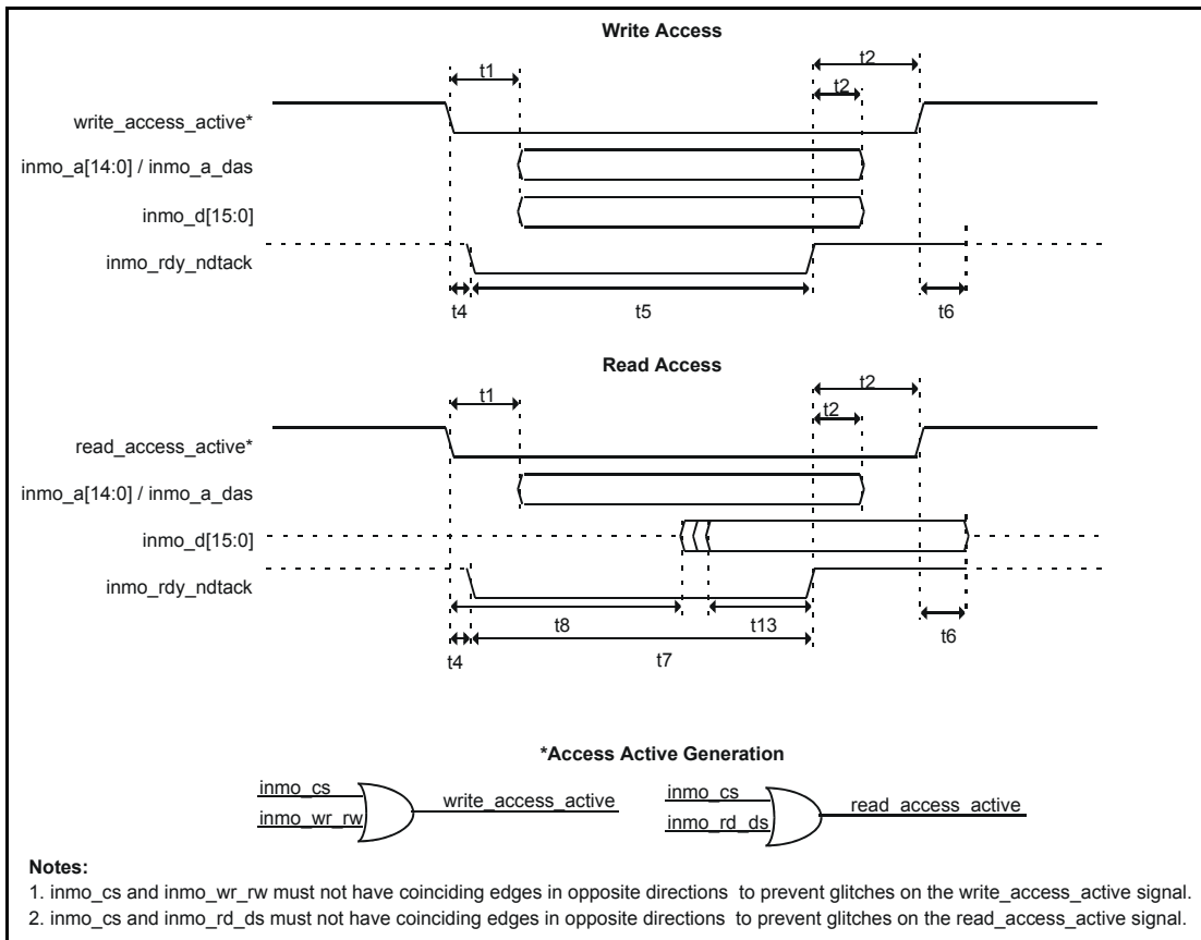
Figure 103 - Non-multiplexed CPU Interface - Intel Mode
