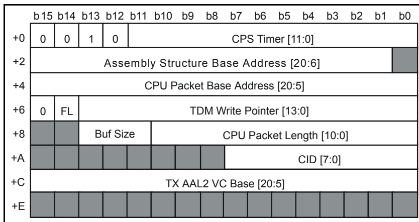
Figure 43 - Assembly Event - Send CPU AAL2 Packet
