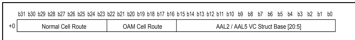
Figure 13 - UTOPIA LUT Entry Format
