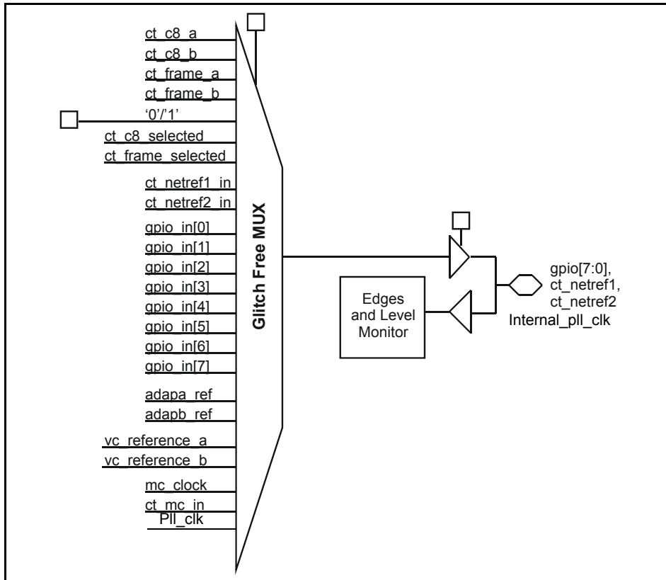
Figure 100 - GPIO Functionality
