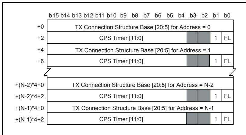
Figure 79 - HDLC Address LUT (AAL2)
