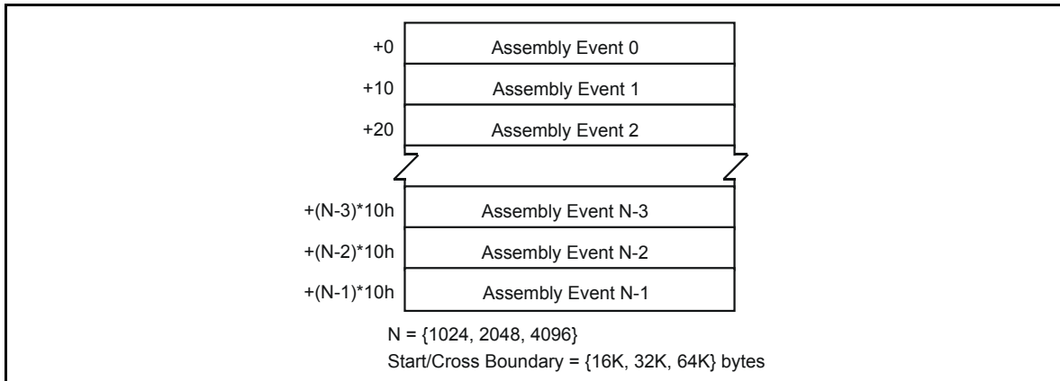
Figure 36 - Assembly Event Queue
