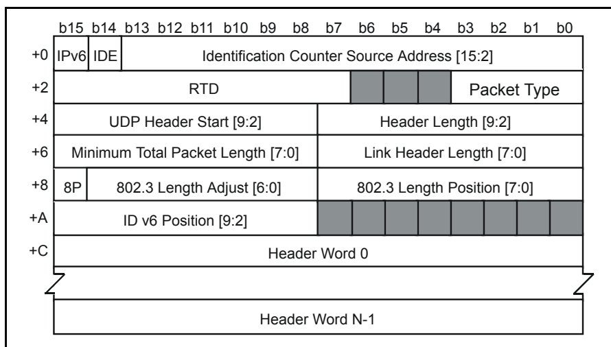
Figure 46 - TX RTP Header Structure
