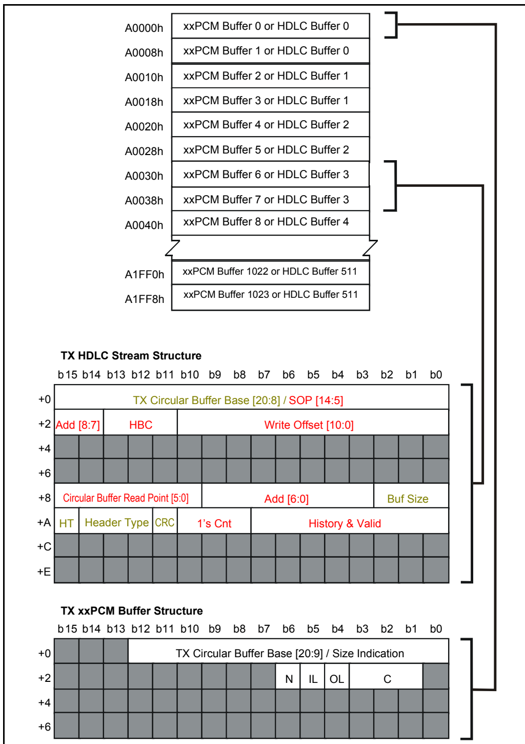
Figure 74 - TX TDM Control Memory
