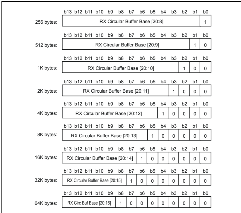
Figure 86 - RX Circular Buffer Base and Size
