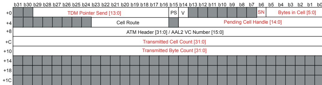
Figure 33 - TX AAL2 VC Structure
