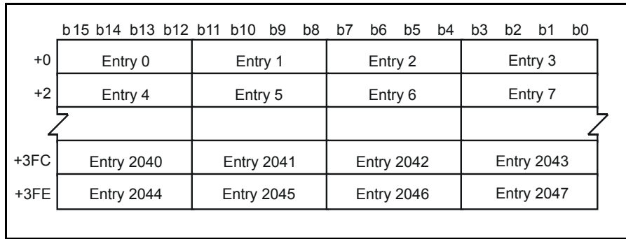
Figure 58 - Generic UUI/LI Table
