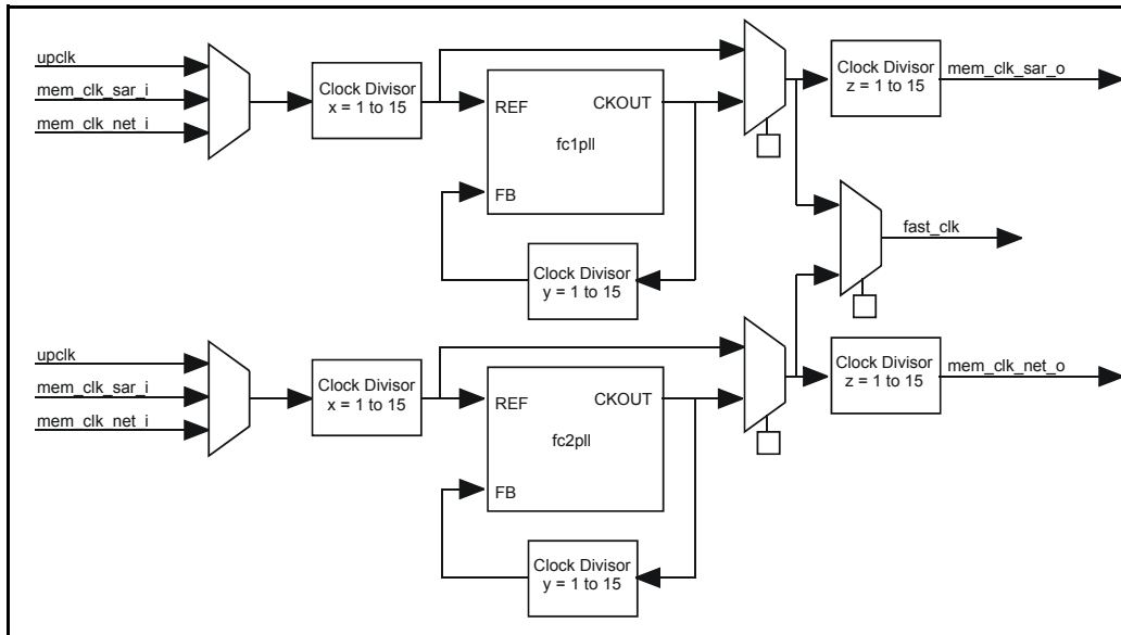
Figure 95 - Clock Synthesis
