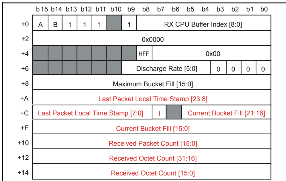
Figure 71 - RX AAL2 CPU Channel Structure
