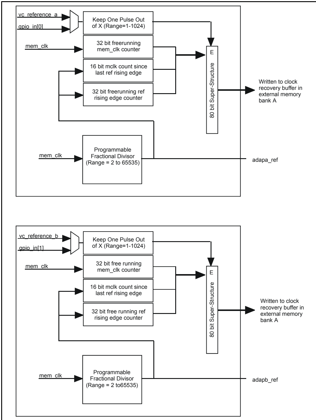
Figure 99 - Adaptive Clock Recovery Modules
