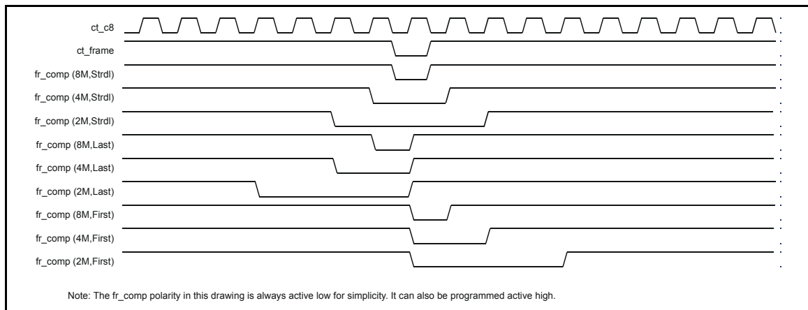
Figure 92 - TDM Bus Timing - fr_comp Generation
