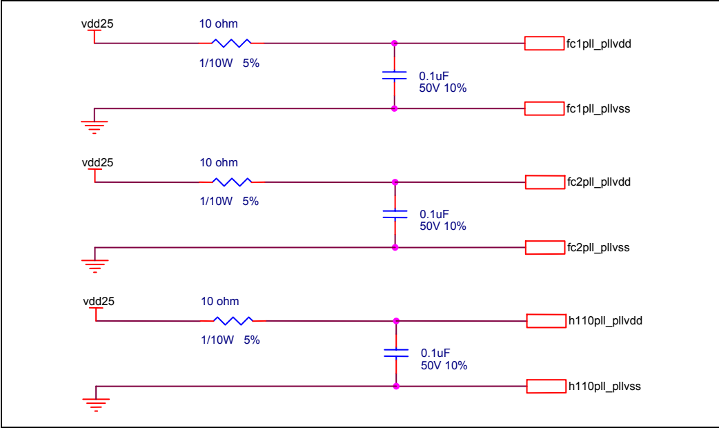
Figure 102 - PLL Noise Reduction Circuits
