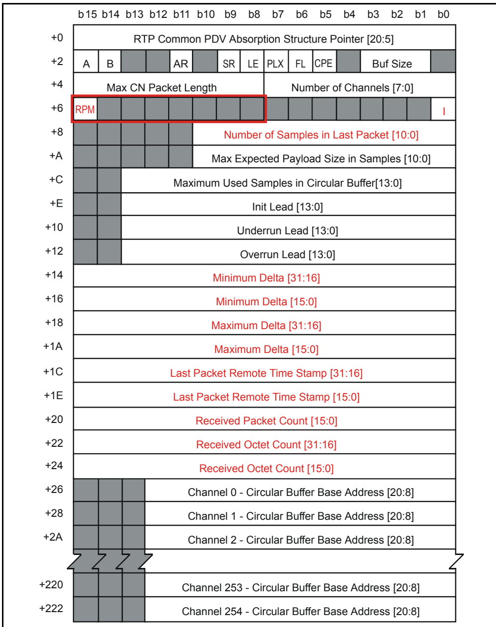
Figure 60 - RX RTP xxPCM Channel Structure
