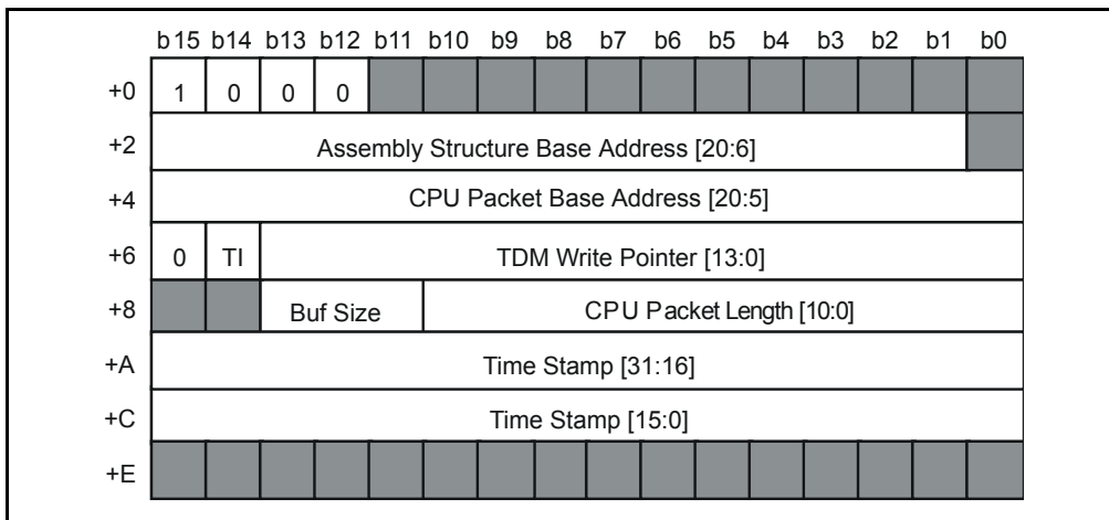
Figure 38 - Assembly Event - Send HDLC RTP Packet
