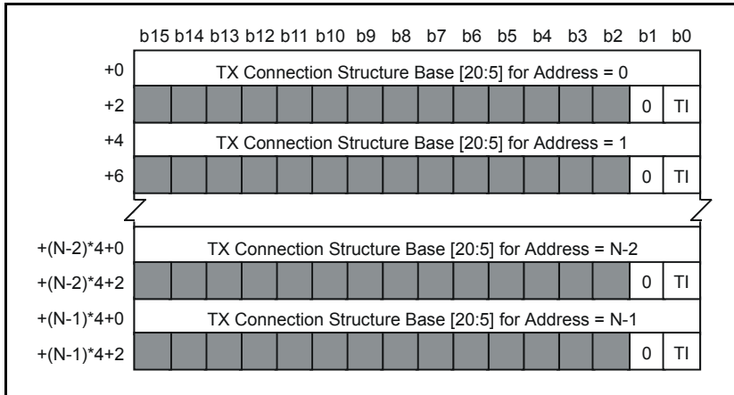
Figure 78 - HDLC Address LUT (RTP)
