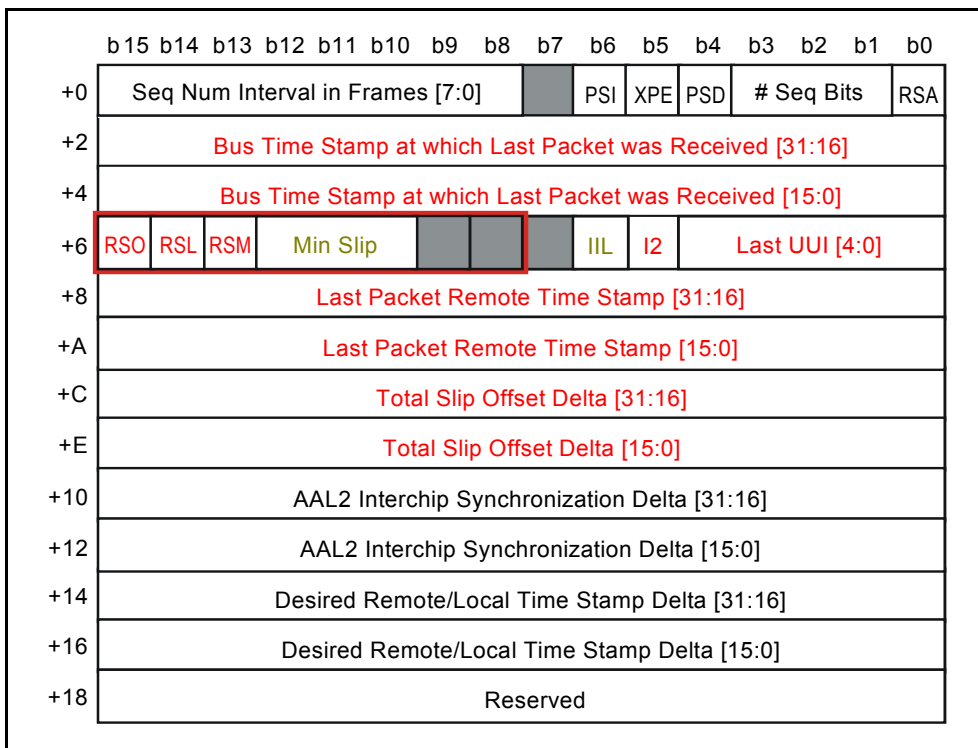
Figure 64 - AAL2 Common PDV Absorption Structure
