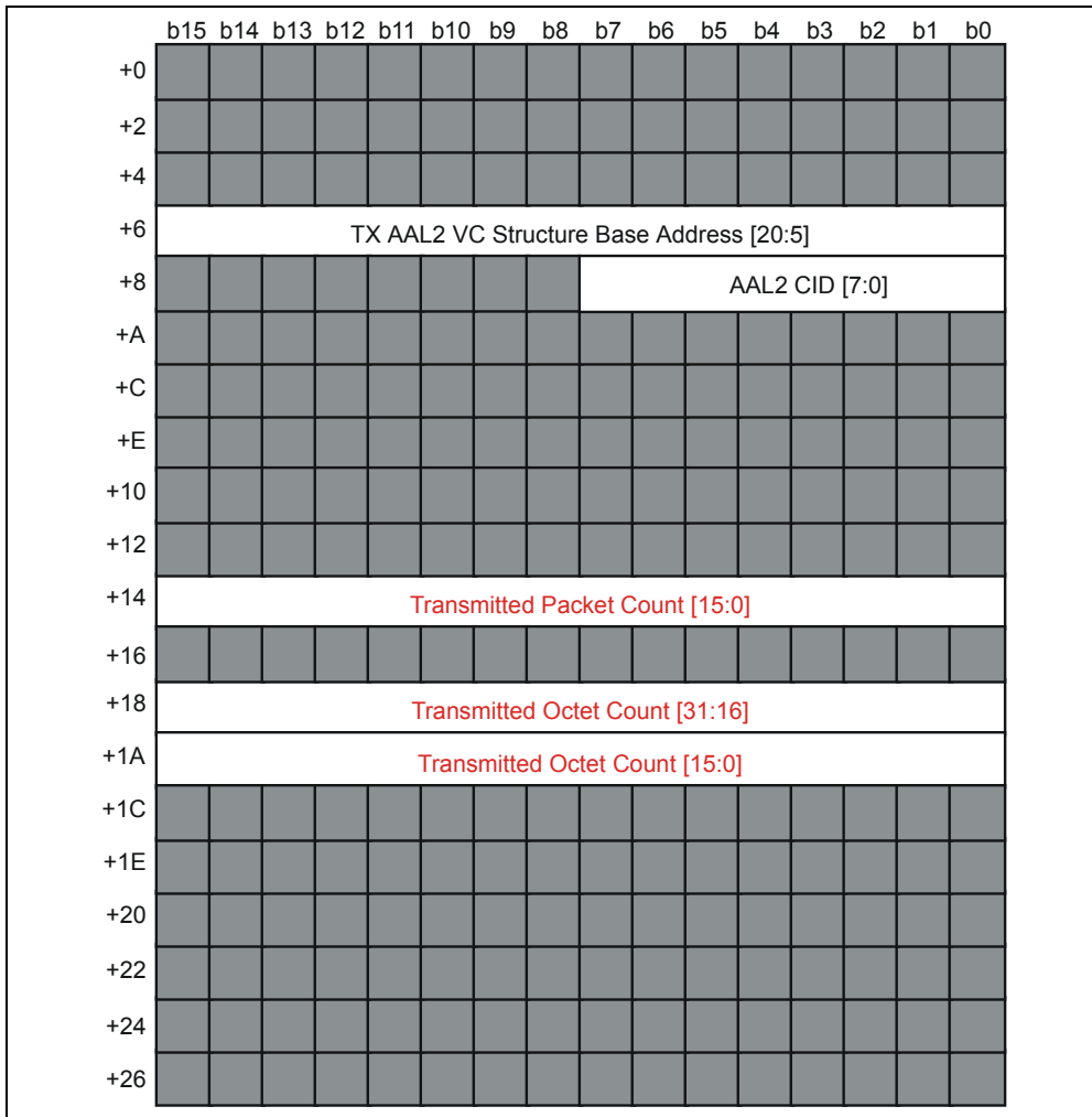
Figure 47 - TX AAL2 Connection Structure
