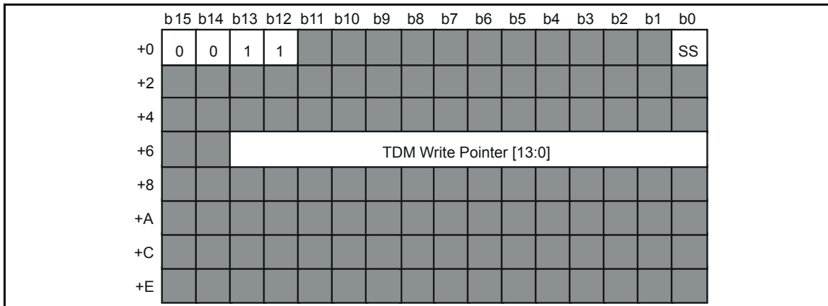
Figure 37 - Assembly Event - Send Start of Frame
