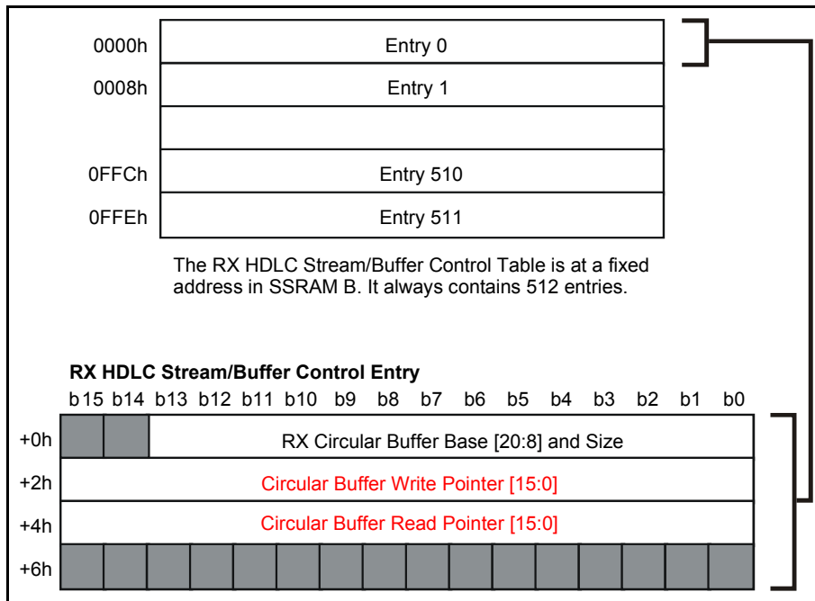
Figure 85 - RX HDLC Stream/Buffer Control Table
