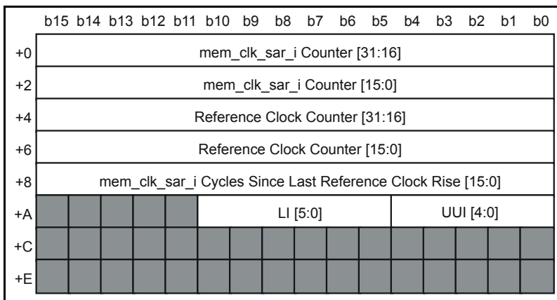
Figure 97 - Adaptive Clock Recovery AAL2 Event Structure
