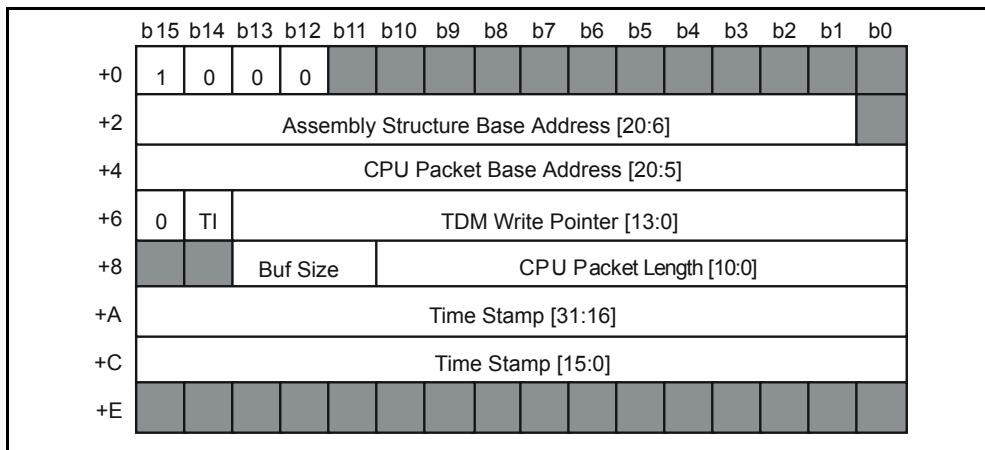
Figure 42 - Assembly Event - Send CPU RTP Packet
