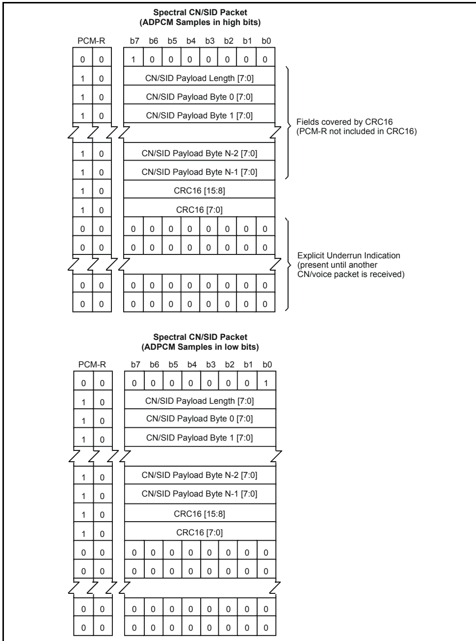
Figure 88 - Format of RX xxPCM TSSTs - 2 of 2
