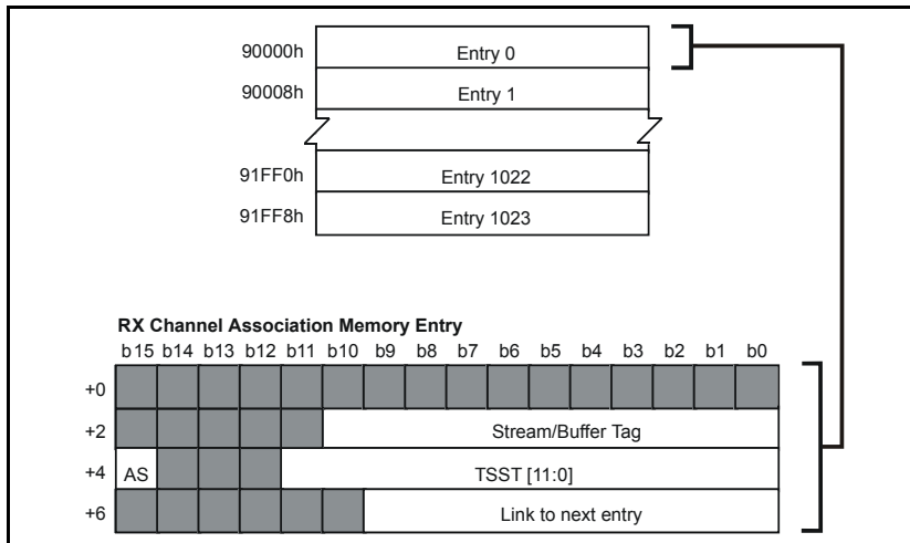
Figure 81 - RX Channel Association Memory
