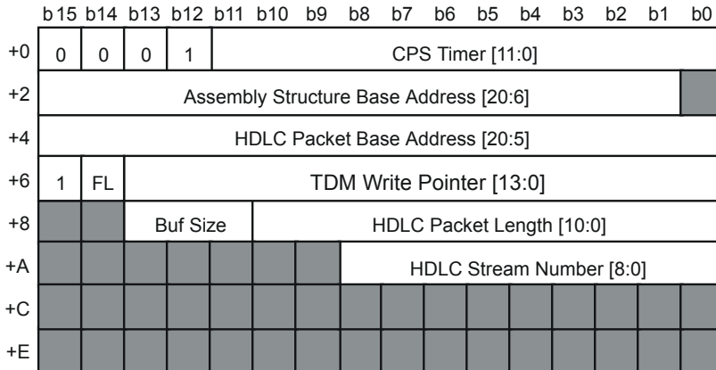
Figure 39 - Assembly Event Send HDLC AAL2 Packet
