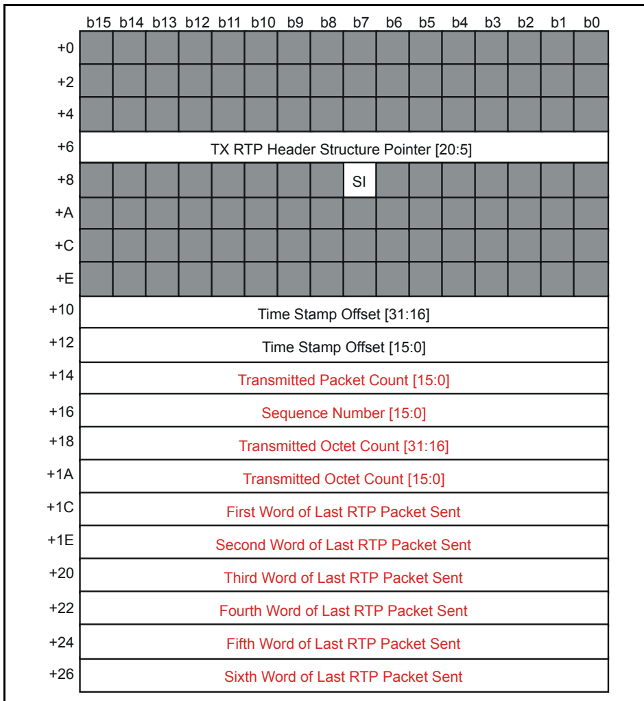
Figure 44 - TX RTP Connection Structure
