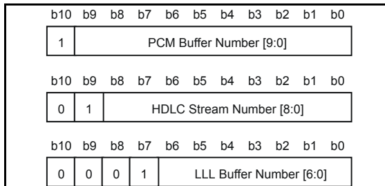
Figure 82 - Stream/Buffer Tag Format
