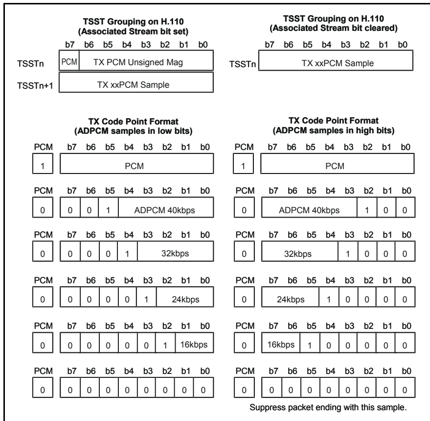
Figure 80 - Format of TX xxPCM TSSTs
