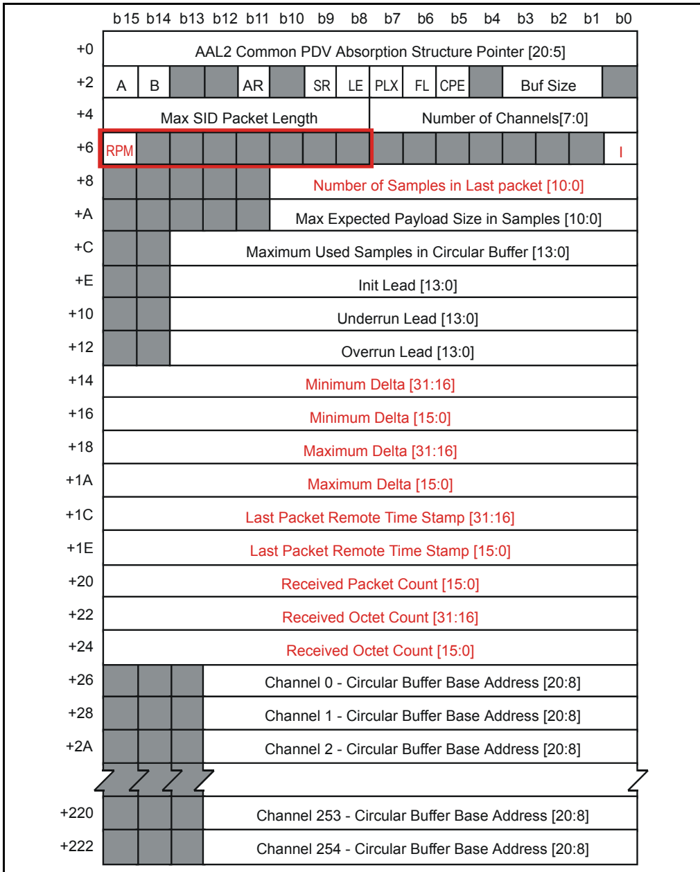
Figure 61 - RX AAL2 xxPCM Channel Structure
