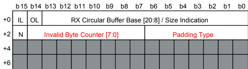
Figure 83 - RX TDM Control Memory
