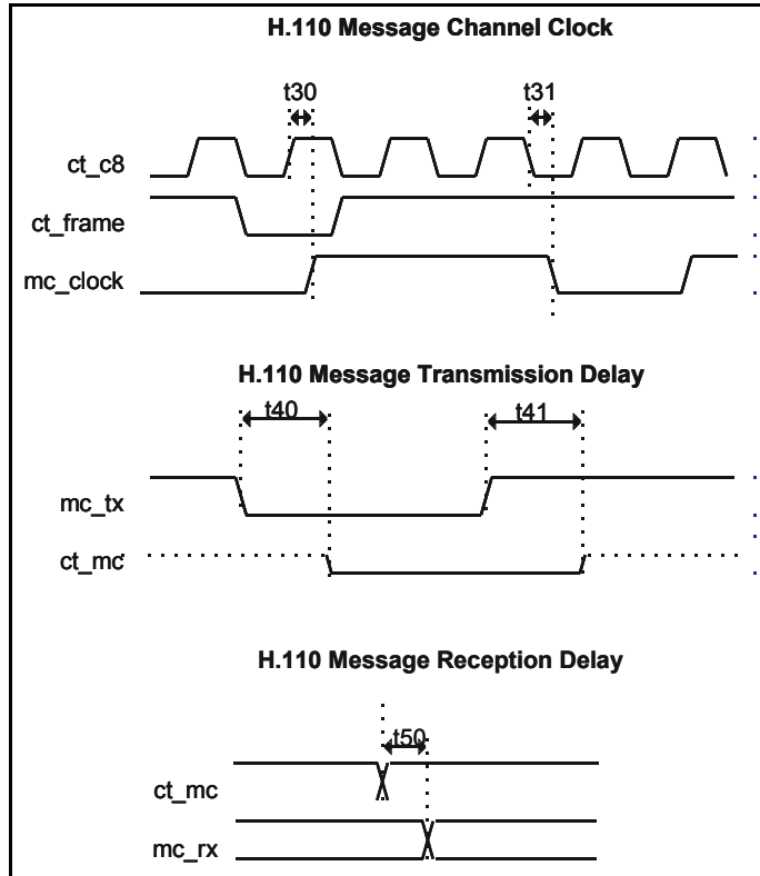
Figure 109 - H.110 Message Handling
