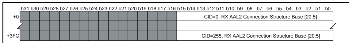
Figure 34 - RX AAL2 CID Translation Structure
