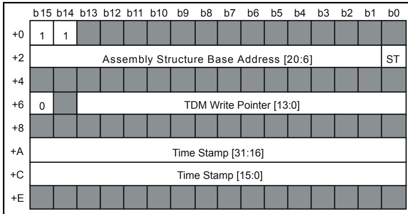
Figure 41 - Assembly Event - Service xxPCM AAL2 Channel
