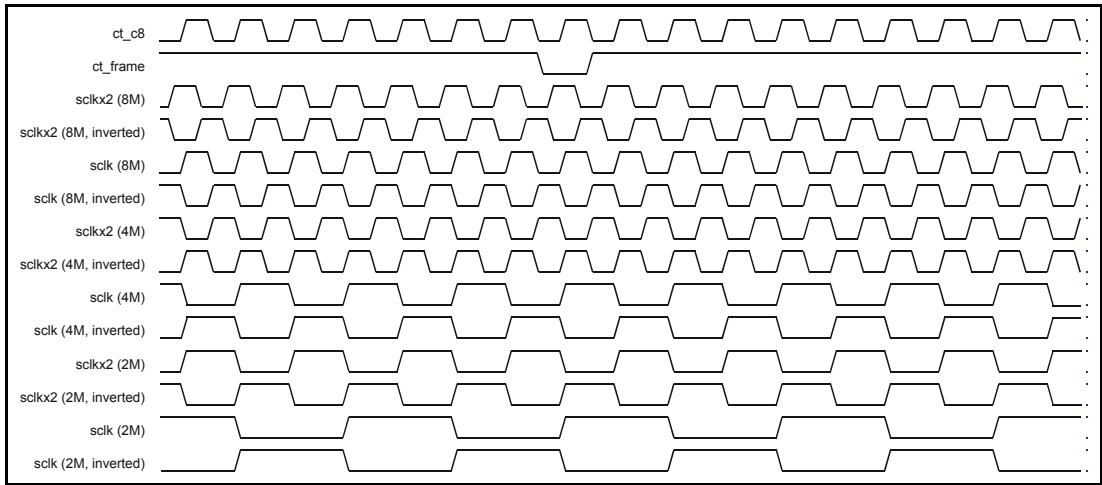
Figure 93 - TDM Bus Timing - sclkx2 Generation
