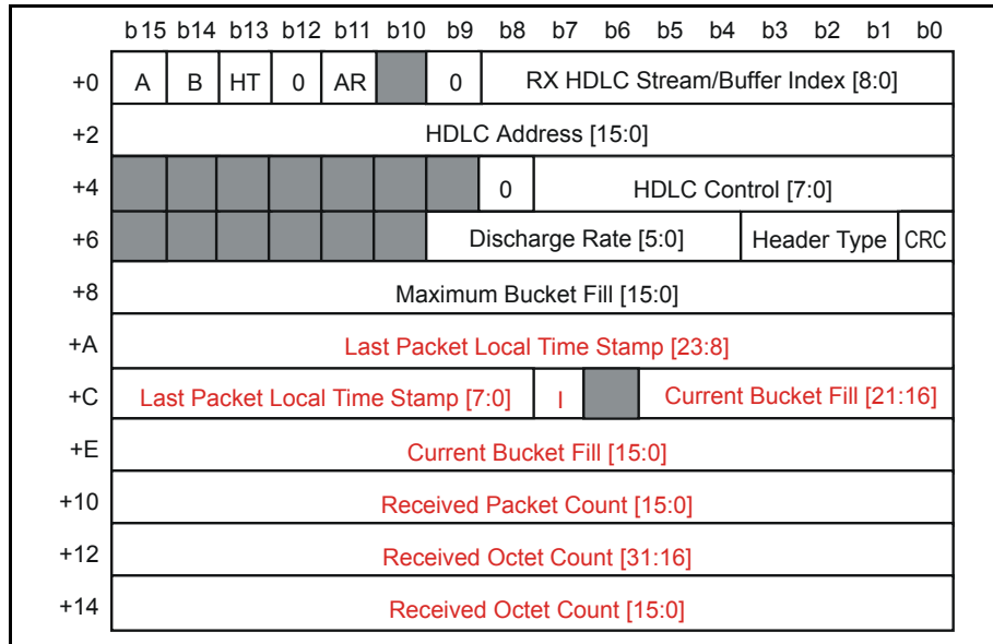
Figure 66 - RX AAL2 HDLC Channel Structure
