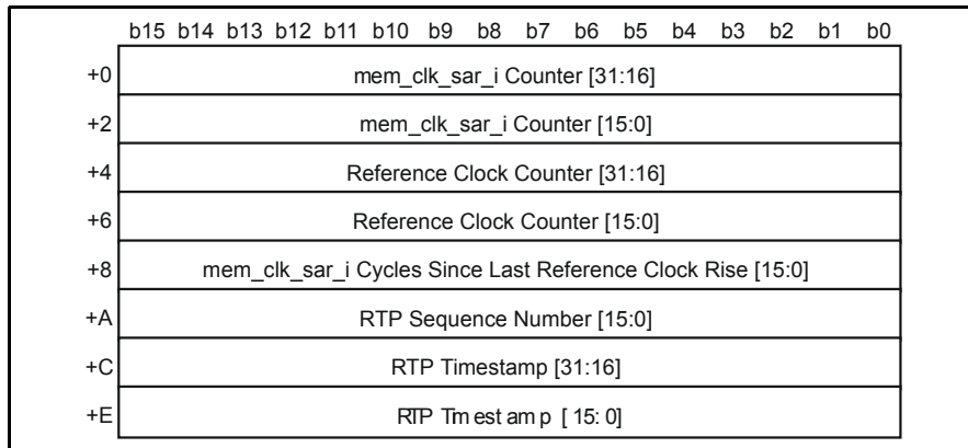
Figure 98 - Adaptive Clock Recovery RTP Event Structure
