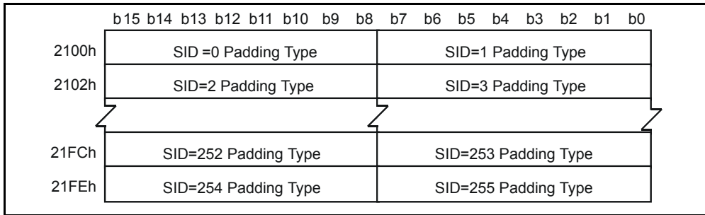
Figure 90 - SID Packet Conversion Lookup Table
