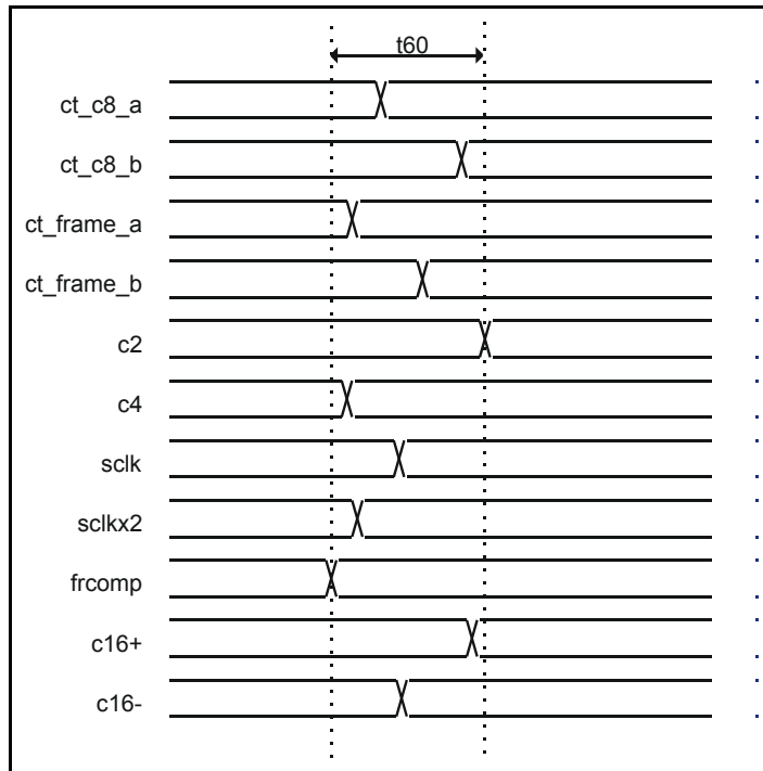
Figure 15.1 - H.110 Clock Skew (when chip is Master)
