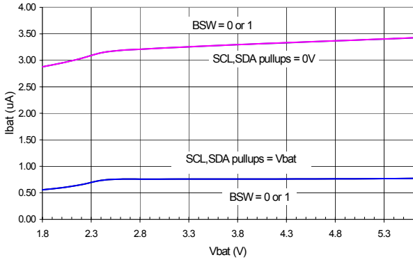
FIGURE 5. I_{BAT} vs V_{BAT} , SIB = 0
