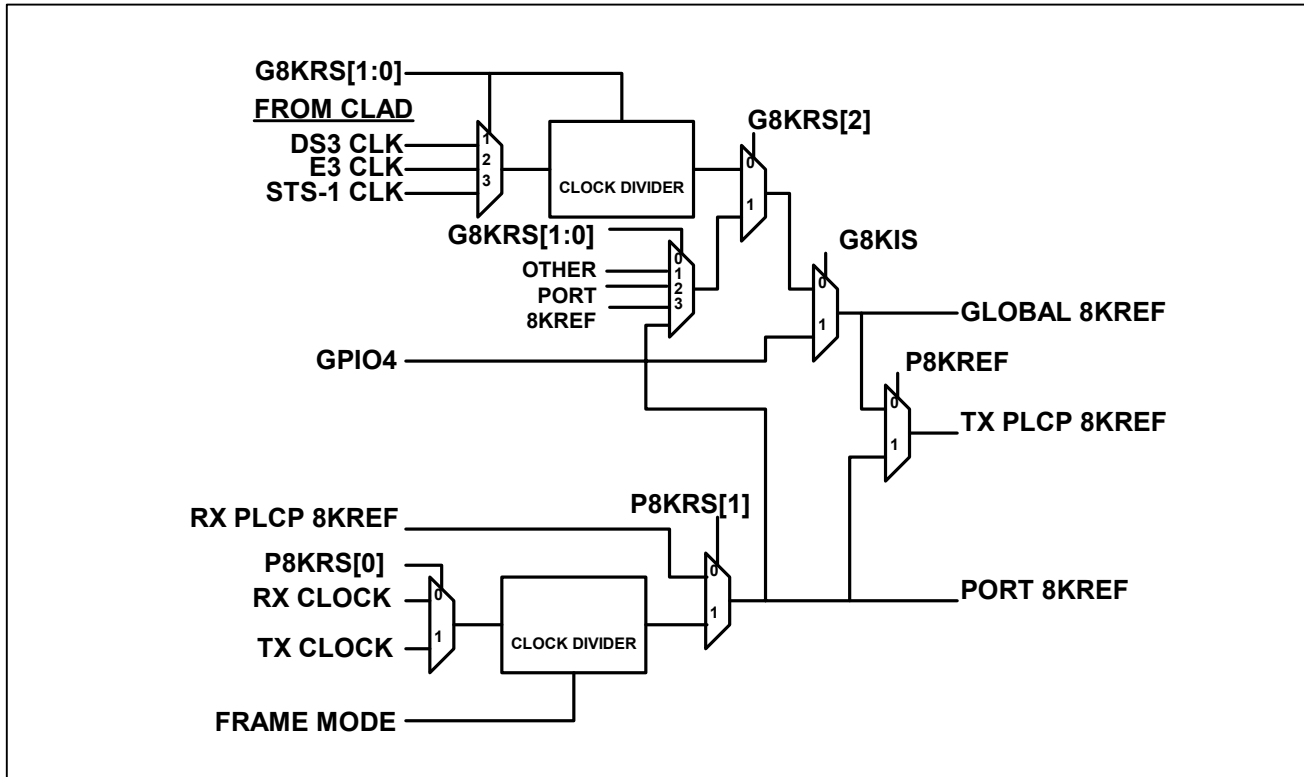
Figure 10-6. 8KREF Logic
